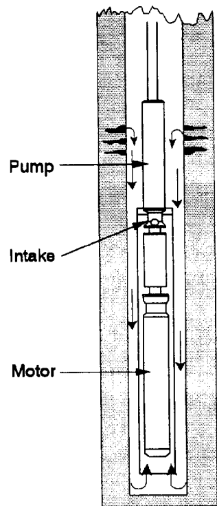
Shrouded ESP Fig. 4
