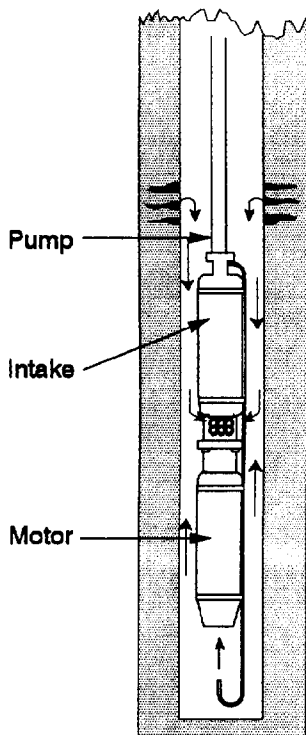
Recirculation Tap Fig. 5
