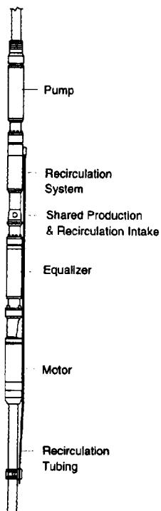
Fig. 7 Single Intake Method
