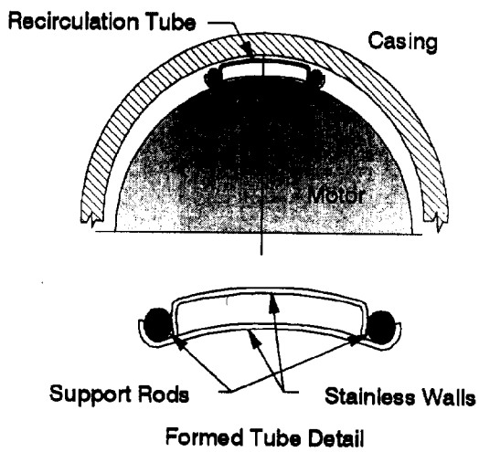
Recirculation Tube Fig. 8
