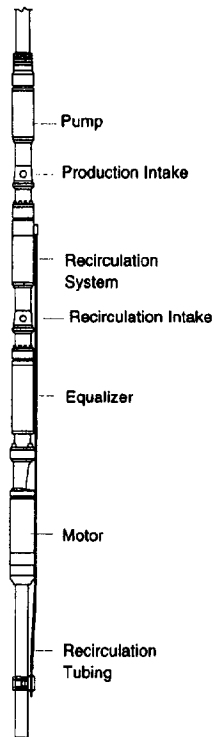
Fig. 6 Double Intake Method
